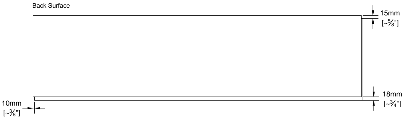
SANDSTONE PANEL DETAIL SCALE: 1" = 1'-0"
