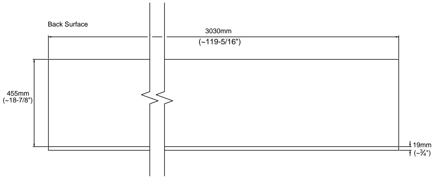
ROUGHSAWN - PANEL DETAIL SCALE: 1" = 1'-0"
