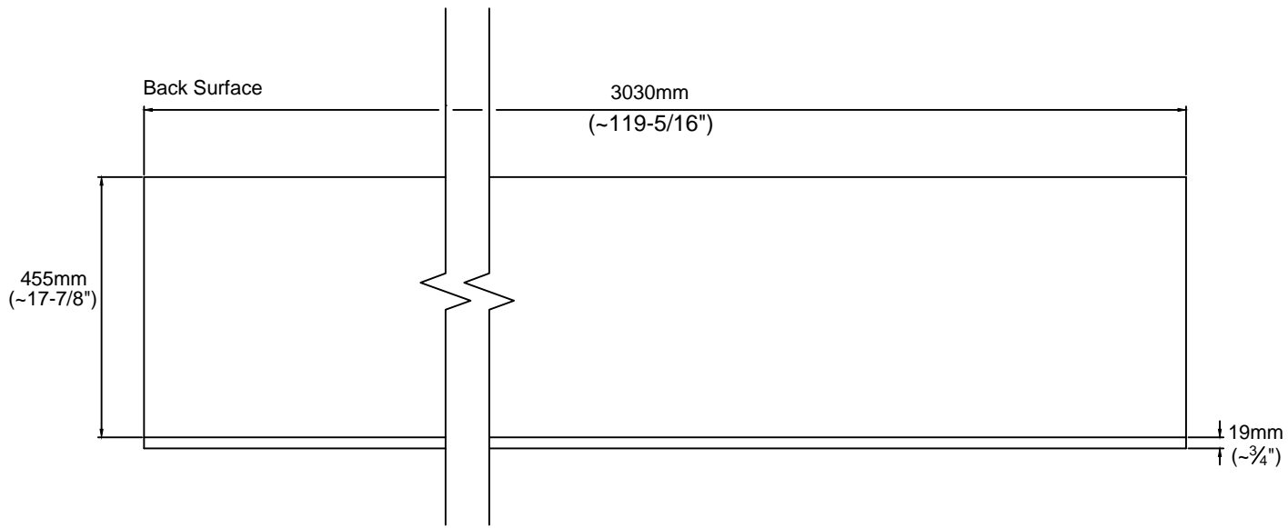
METALLIC - RIBBED - PANEL DETAIL SCALE: 1" = 1'-0"
