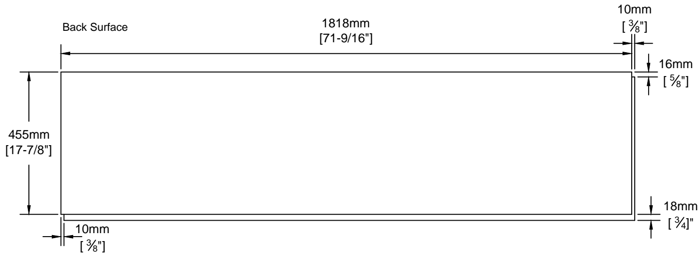
CANYON BRICK PANEL DETAIL SCALE: 1" = 1'-0"
