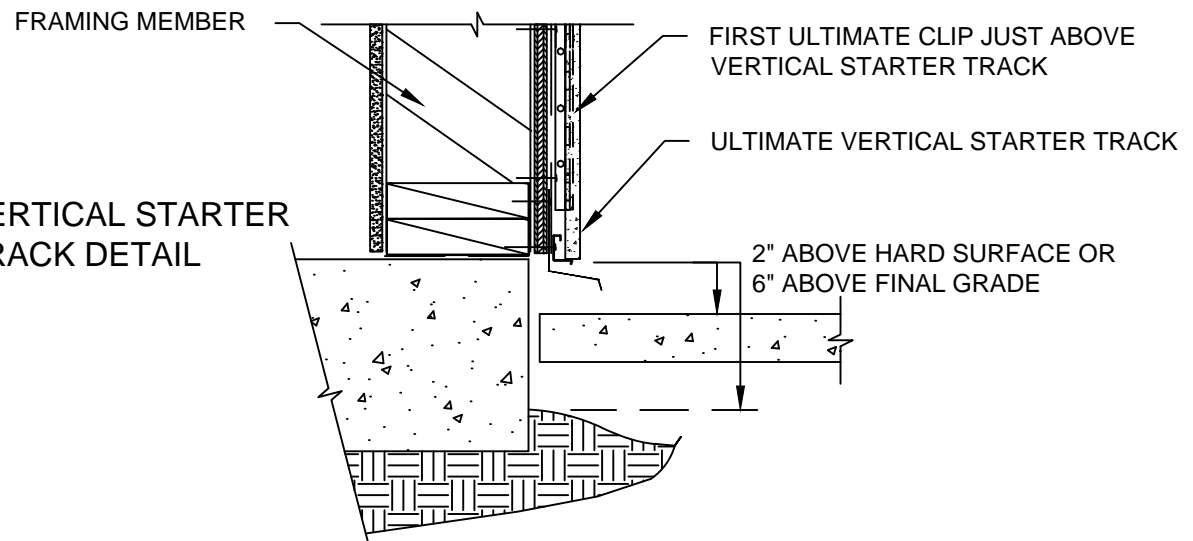
AWP-3030 VERTICAL WITH HORIZONTAL PANEL BAND - TRANSITION DETAIL
