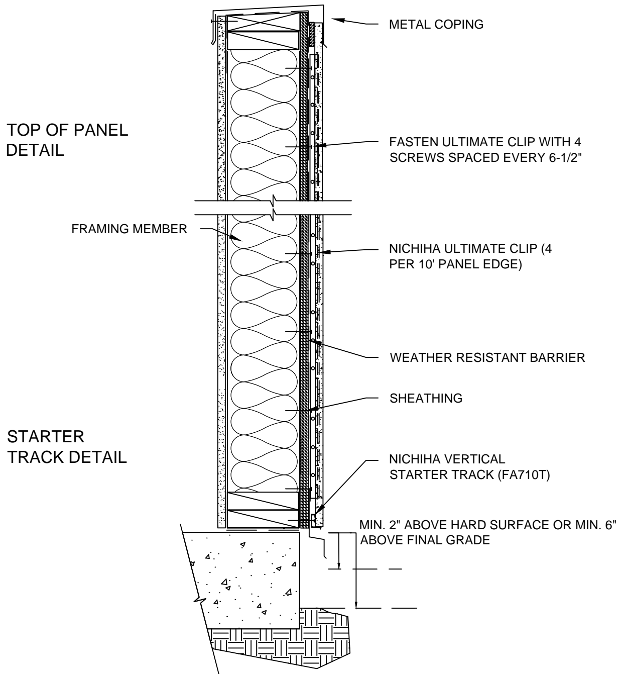
10MM - 10 FOOT VERTICAL PANEL - TYPICAL WALL DETAIL - PARAPET SCALE: 1 1/2" = 1'-0"
