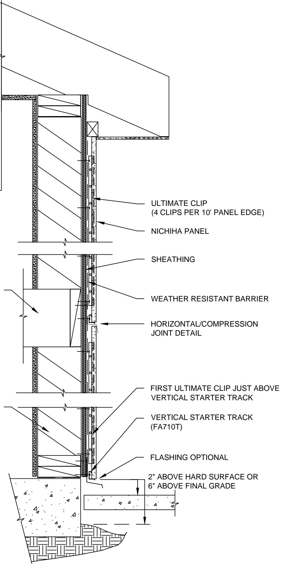
10MM - STANDARD - 10' VERTICAL PANEL - TYPICAL WALL DETAIL
