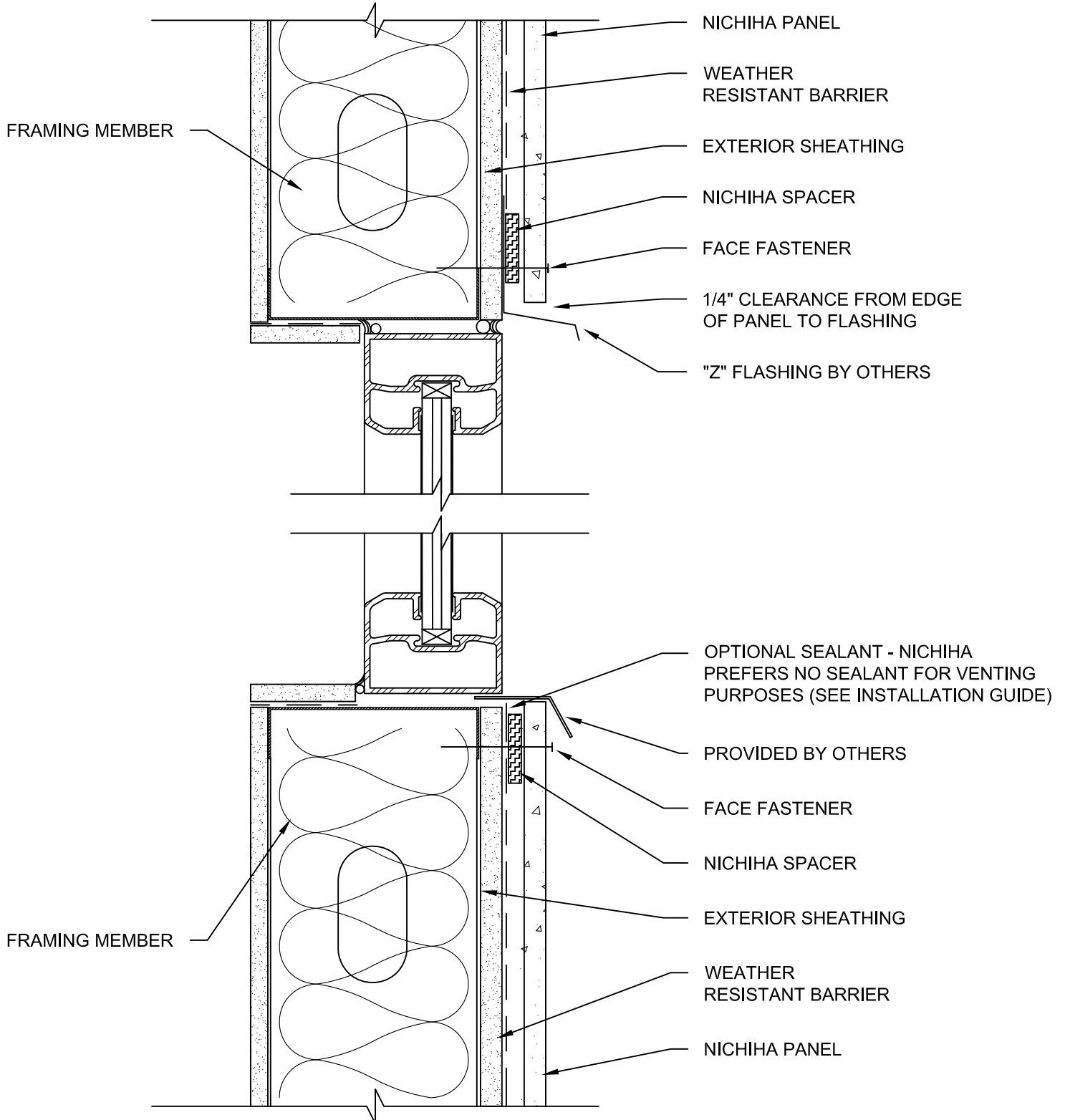
10 mm - METAL STUD PANEL STOREFRONT WINDOW HEADER & SILL DETAIL WITH FLASHING
