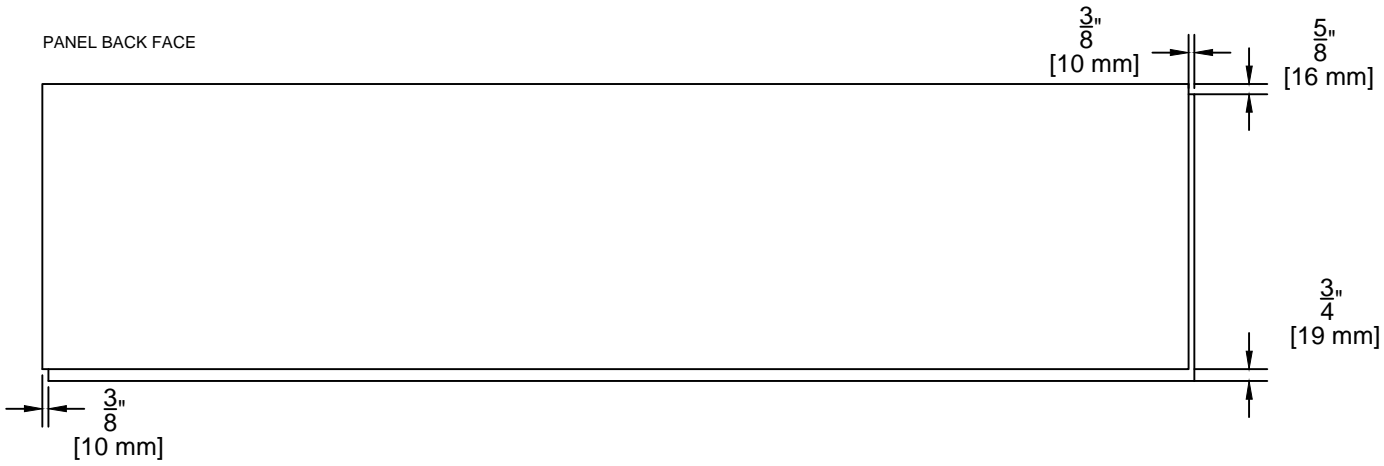
CINDERBLOCK PANEL DETAIL SCALE: 1" = 1'-0"
