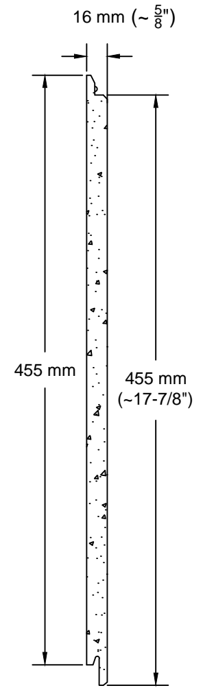
PANEL SECTION
