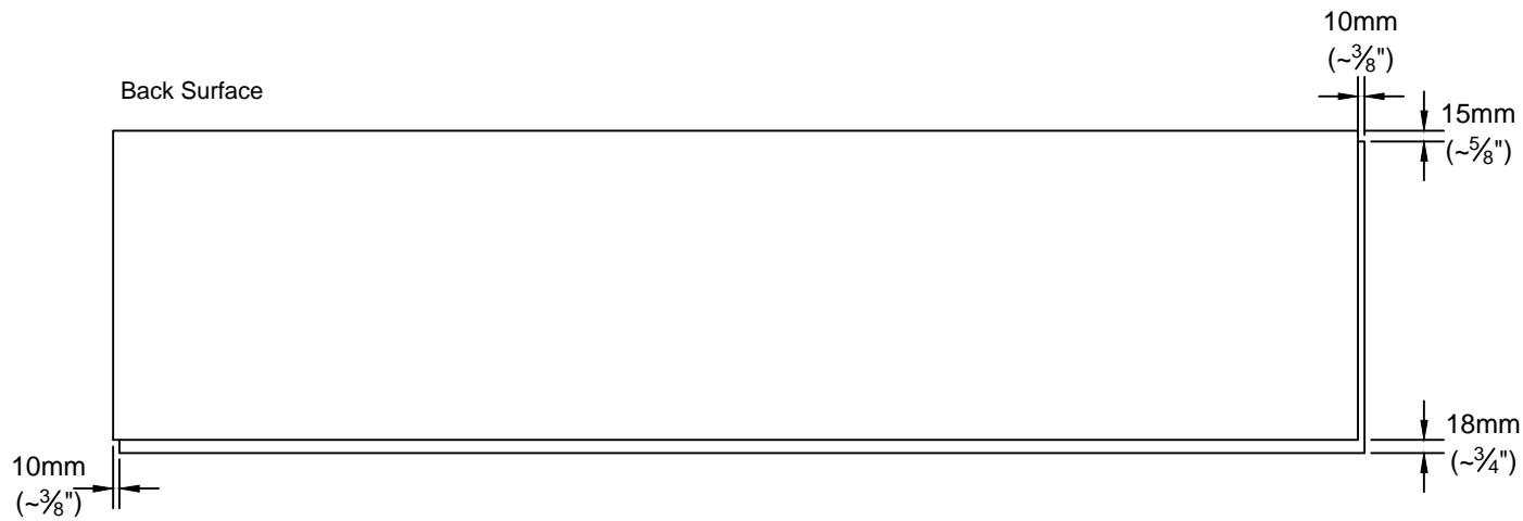
ARCHITECTURAL BLOCK (LARGE) PANEL DETAIL SCALE: 1" = 1'-0"
