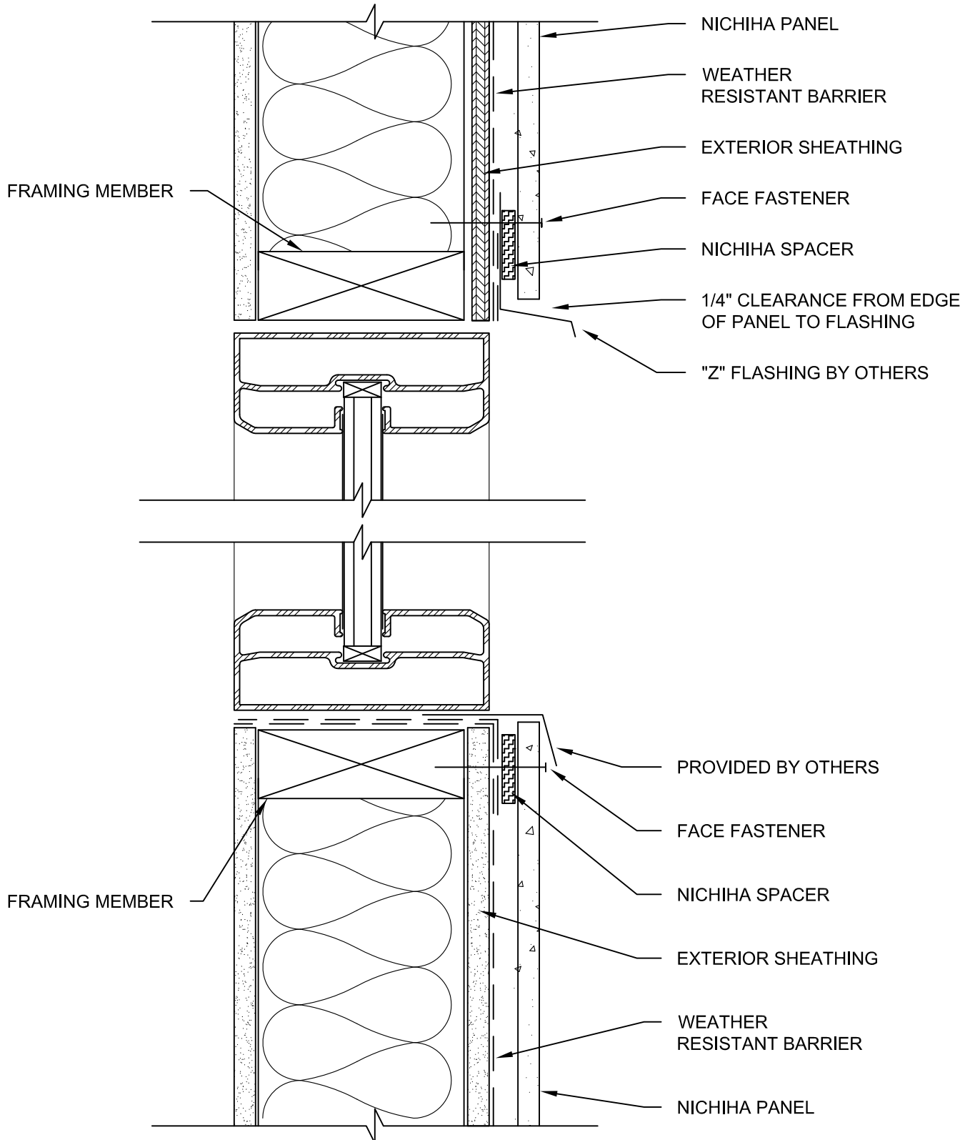
10 mm WOOD STUD PANEL RECESSED WINDOW HEADER & SILL DETAIL WITH FLASHING
