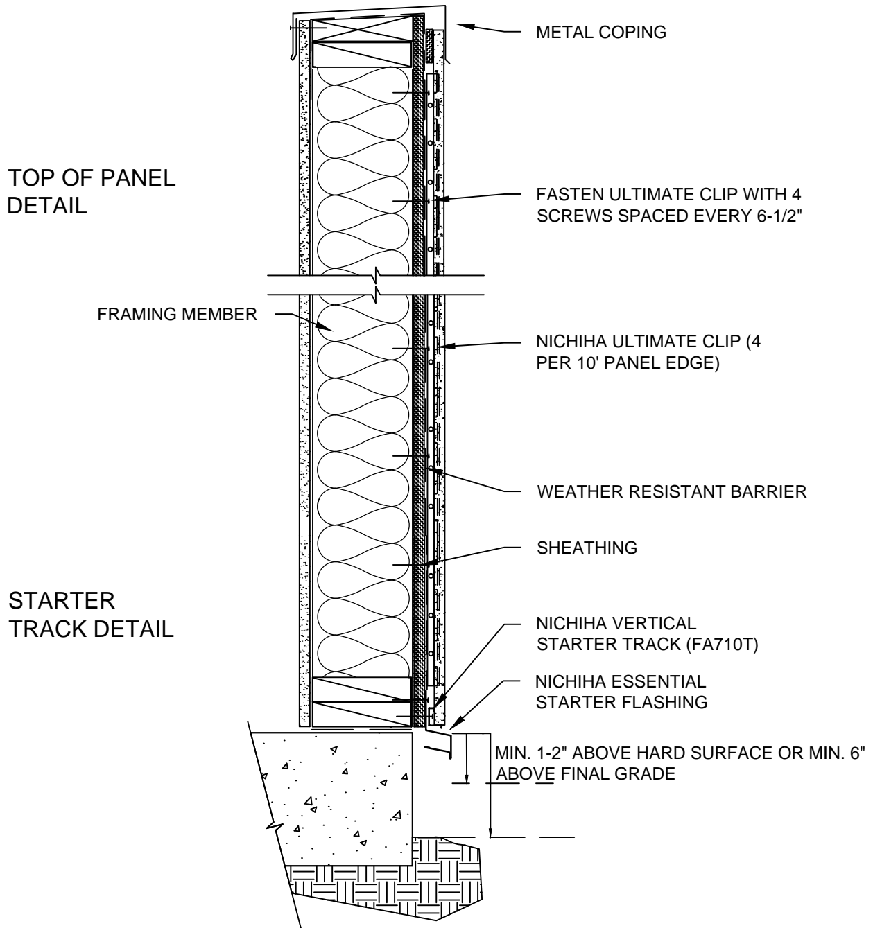
10MM - 10 FOOT VERTICAL PANEL - TYPICAL WALL DETAIL - PARAPET SCALE: 1 1/2" = 1'-0"
