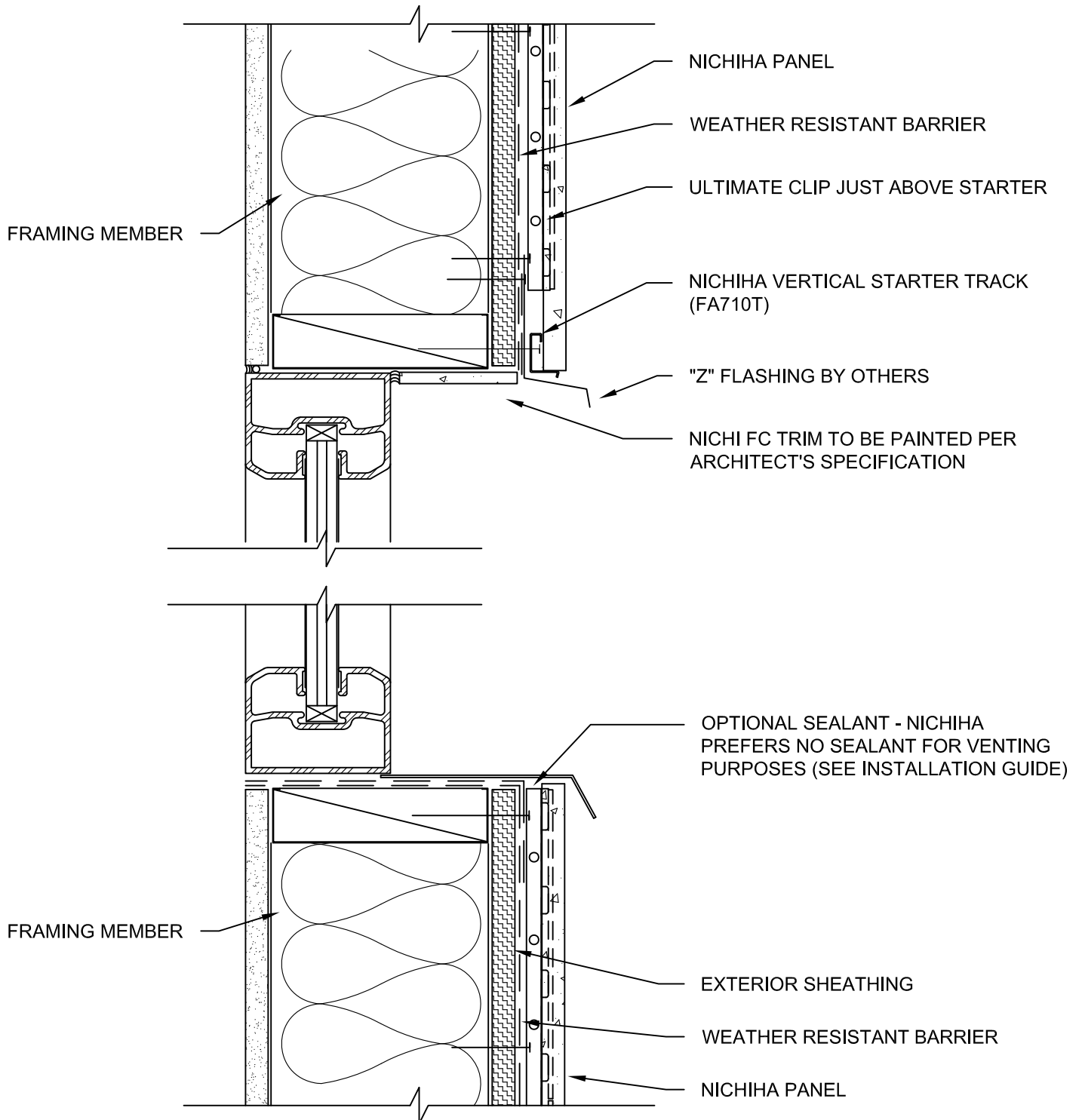
10MM - 10' VERTICAL PANEL - RECESSED WINDOW HEADER & SILL DETAIL WITH RETURN AS FC SOFFIT & FLASHING
