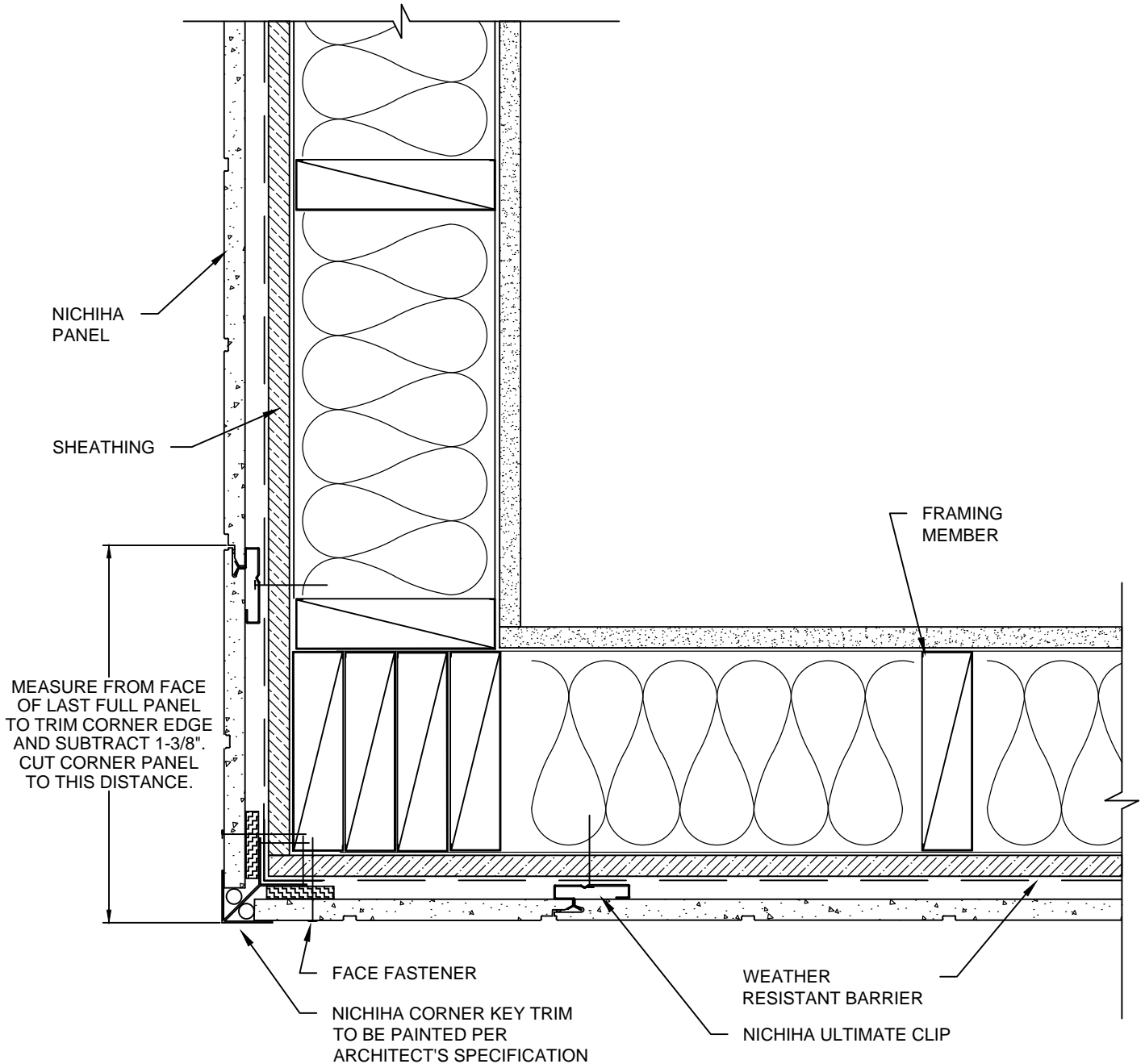
10MM - STANDARD - 10' PANEL VERTICAL - OUTSIDE CORNER DETAIL - NICHHA CORNER KEY TRIM
