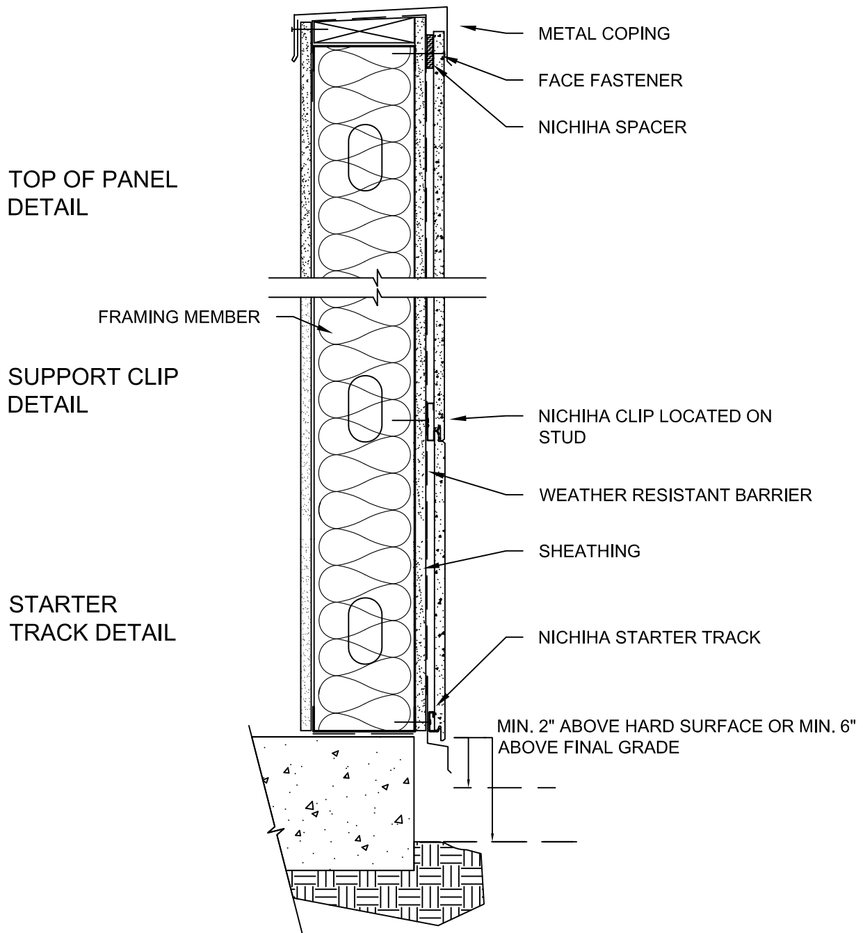
10 mm - METAL STUD PANEL TYPICAL WALL DETAIL WITH PARAPET
