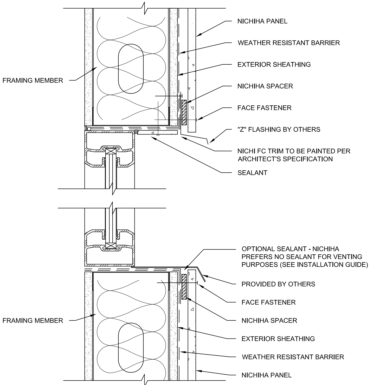
10 mm - METAL STUD PANEL RECESSED WINDOW HEADER & SILL DETAIL WITH RETURN AS FC SOFFIT & FLASHING
