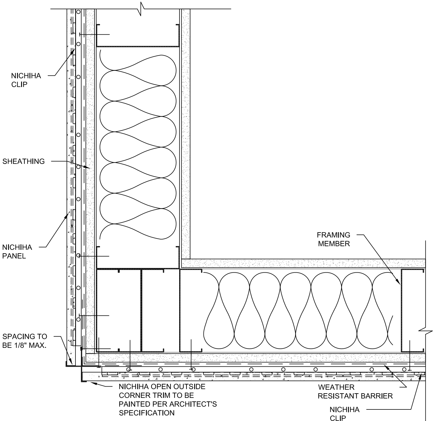
10 mm METAL STUD PANEL OUTSIDE CORNER DETAIL - NICHIIHA OPEN OUTSIDE CORNER TRIM
