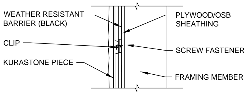
KURASTONE HORIZONTAL JOINT - SECTION
