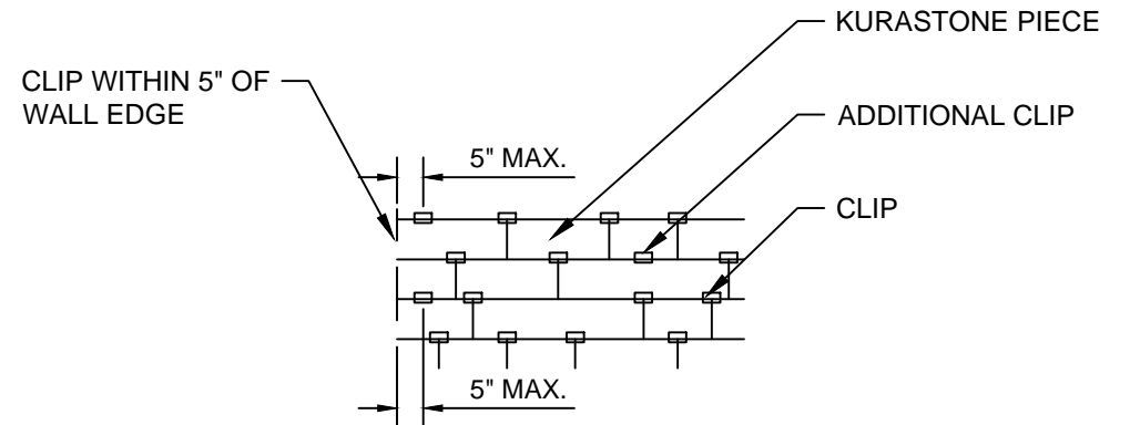
CLIP LOCATION DIAGRAM: NTS
