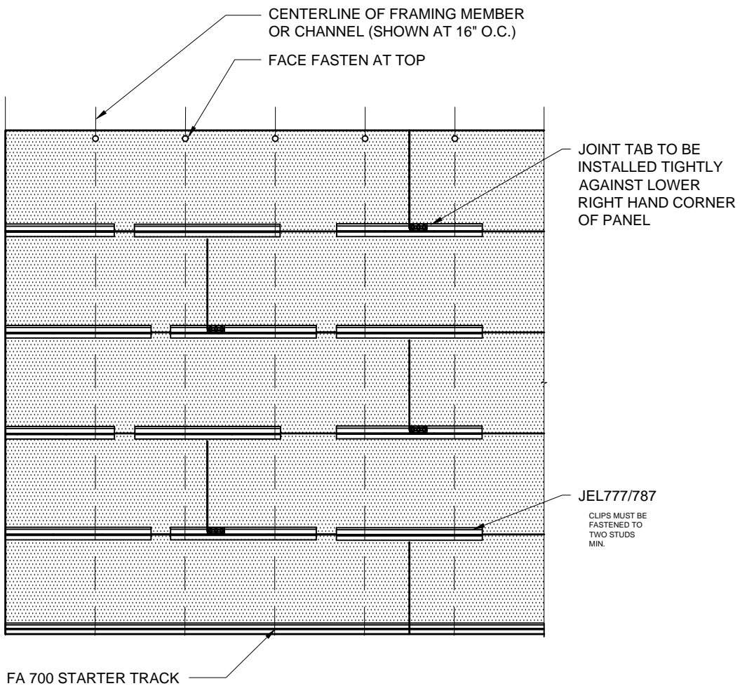
CLIP PLACEMENT FOR STAGGERED PANEL LAYOUT SCALE: 1/2" = 1'-0"
