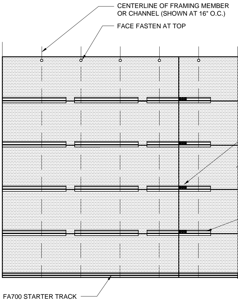
CLIP PLACEMENT FOR STACKED PANEL LAYOUT SCALE: 1/2" = 1'-0"
