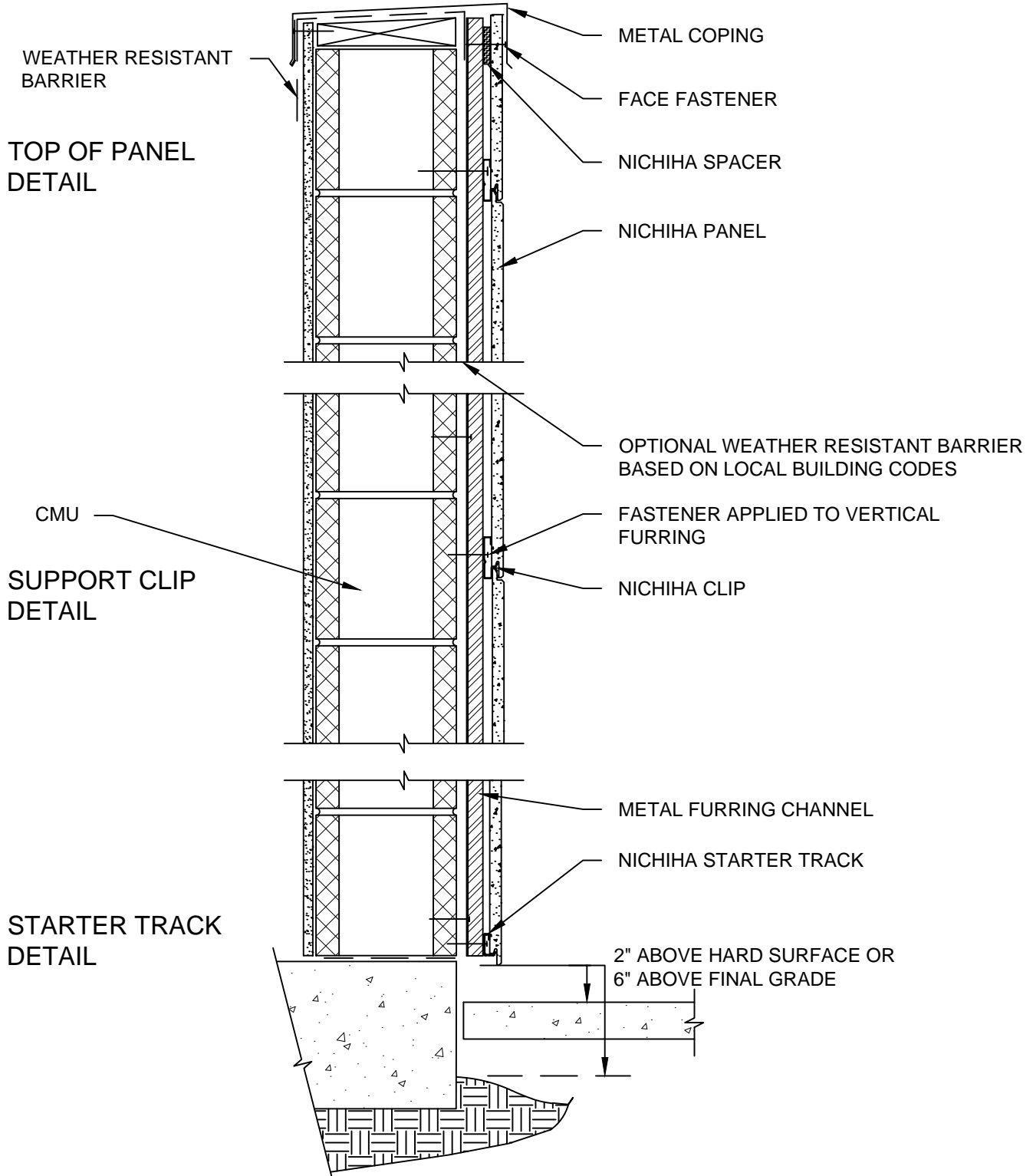
10 mm CMU WITH FURRING 6' & 10' HORIZONTAL PANEL TYPICAL WALL DETAIL
